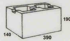
15.42 CHANNEL
